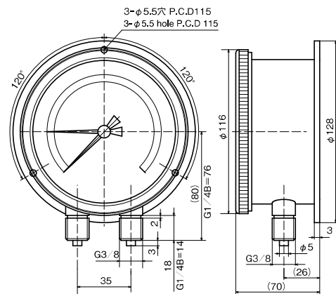
複針ゲージ B型 FA12 WA-4(屋外仕様) Duplex pressure gauge B type FA12 WA-4 (Outdoor specifications)
